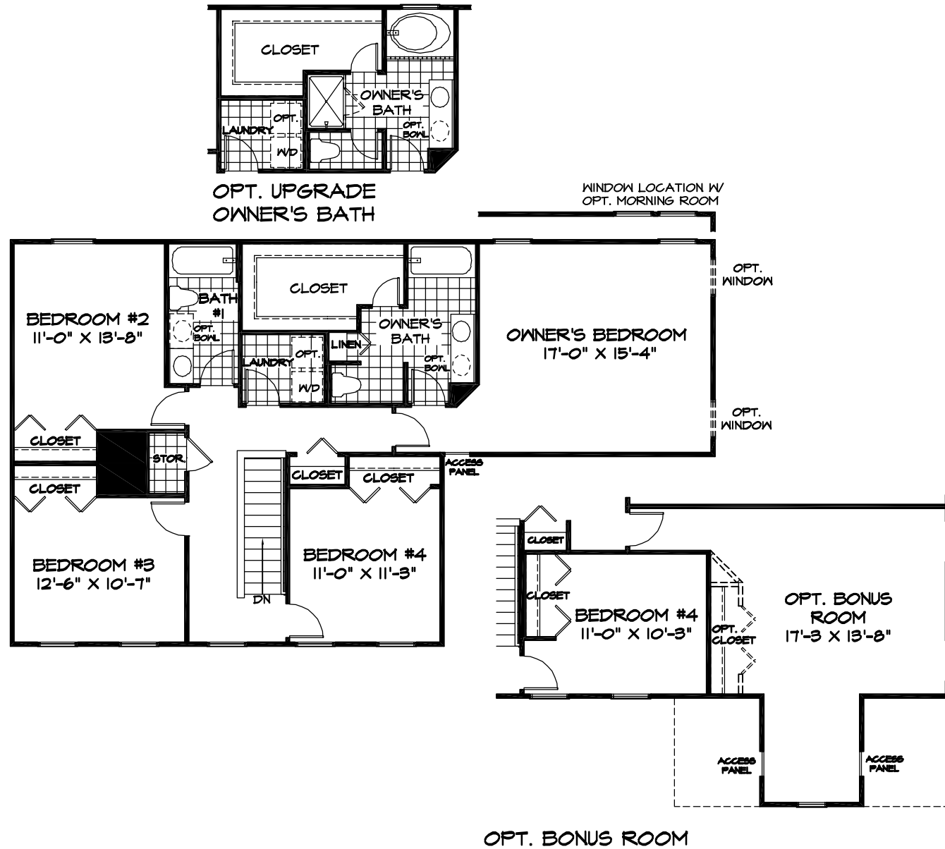
UPPER LEVEL ELEVATION B
